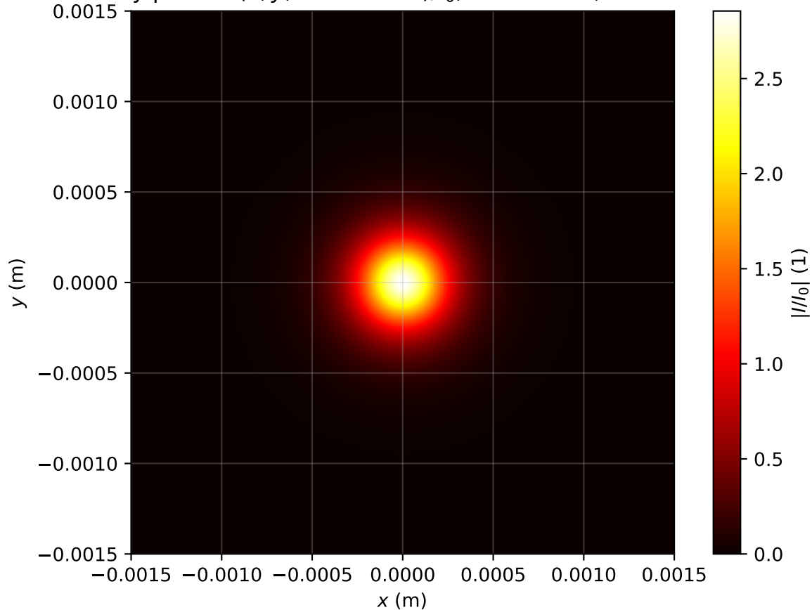
Intensity profile I(x, y, z = 3.344m)/I_0 , P_{in}=1.0P_{cr} , artificial time
